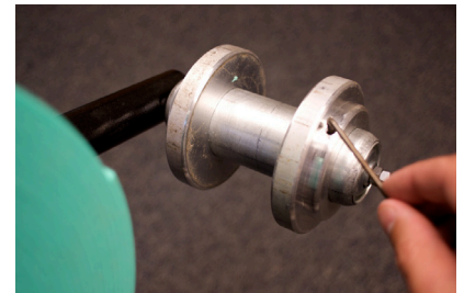
Adjust applicator with 1/8" Allen wrench to fit joist flanges
